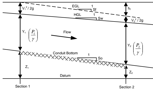
Figure 1: Terms Used in the Energy Equation
