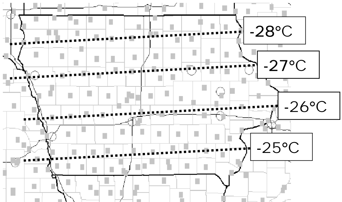
Figure 2: Low (1-day) Pavement Temperature at 98% Reliability
