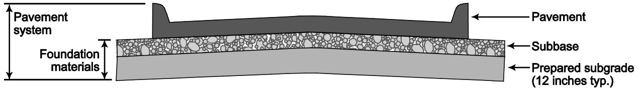
Figure 1: Typical section
