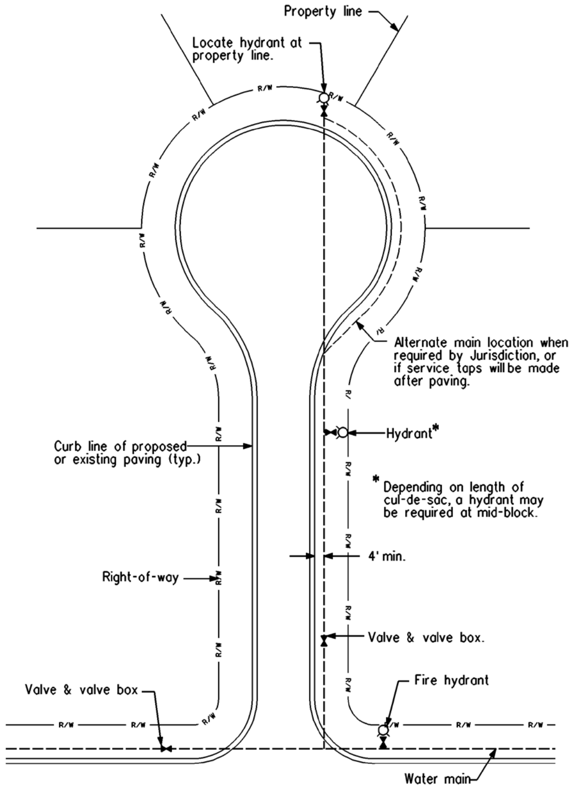
Figure 2: Standard water main location at cul-de-sac
