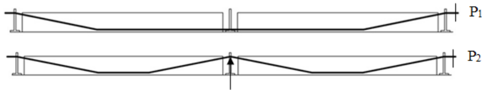
Figure 5.10. Initial and final positions of the harped prestressing strands when tensioning
