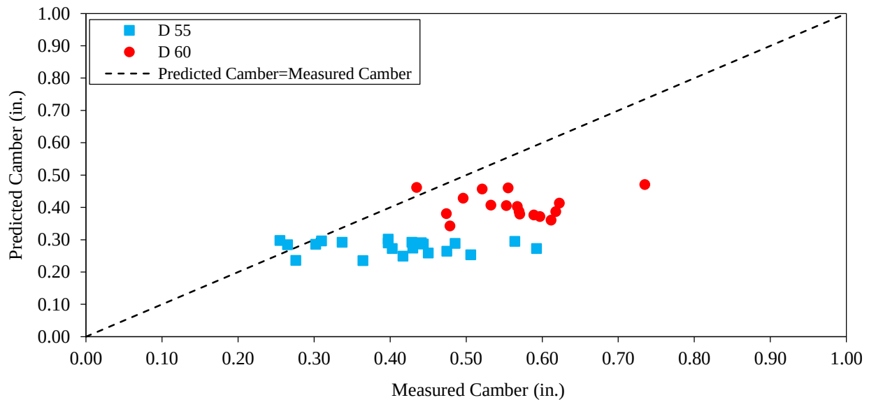
Figure 7.18. Predicted camber versus measured camber using the continuous power function with a zero temperature difference for the small-camber PPCBs
