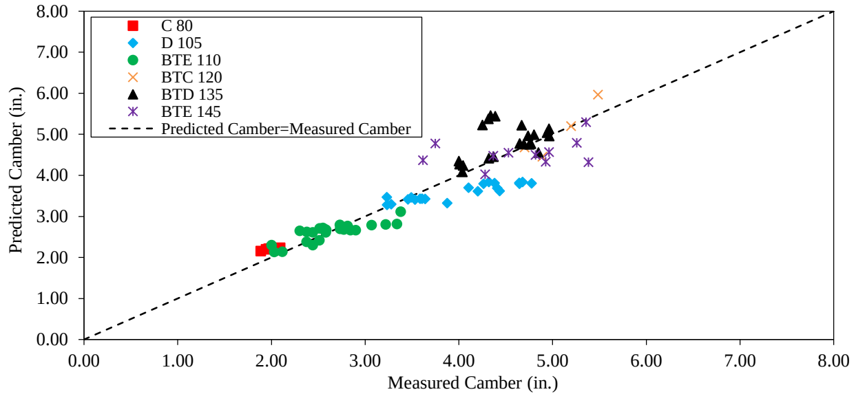
Figure 7.17. Predicted camber versus measured camber using the continuous power function with a 15°F temperature difference for the large-camber PPCBs
