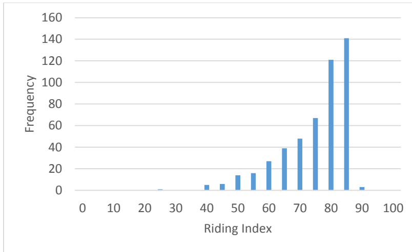
Figure 15. Riding Index for composite built on old CRC Type 3B
