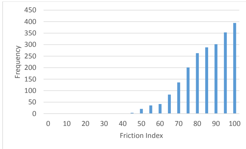
Figure 27. Friction Index for PCC Type 1-Primary
