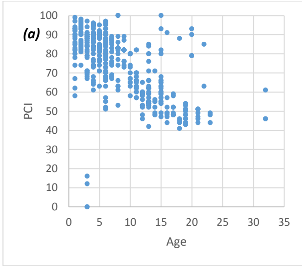
Figure 51. Deterioration of pavement condition by pavement by age for Type 3B composite built on old CRC: (a) using PCI, (b) using PCI-2
