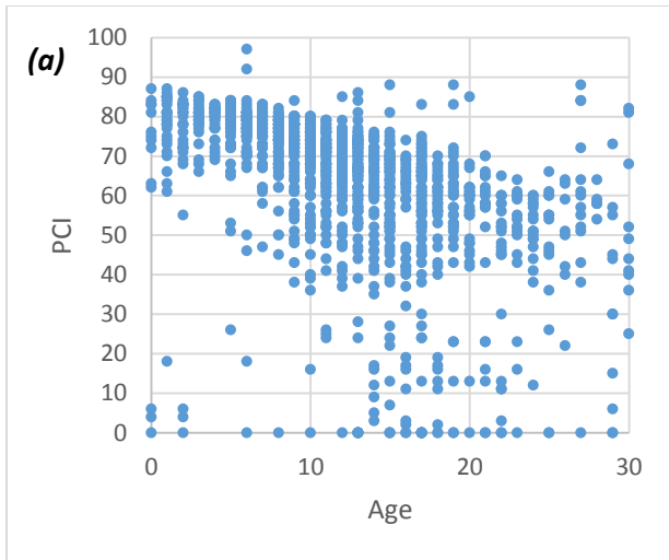
Figure 53. Deterioration of pavement condition by pavement age for AC Type 4-Primary: (a) using PCI, (b) using PCI-2
