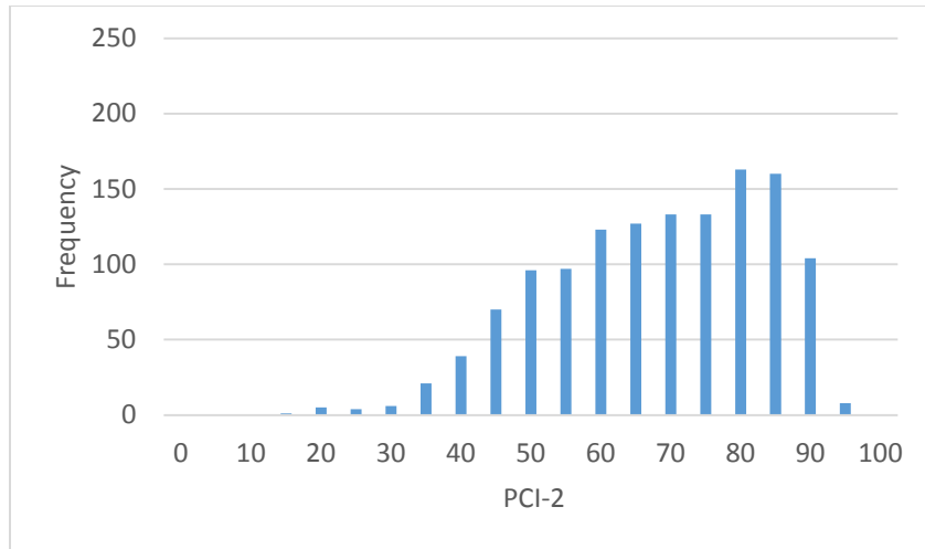
Figure 39. PCI-2 for AC Type 4-Primary
