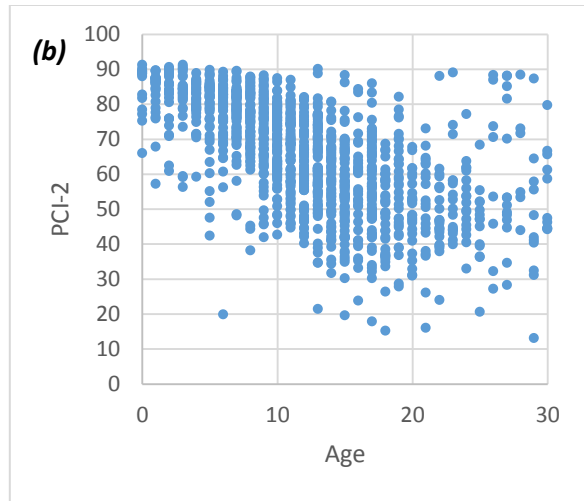
Figure 53. Deterioration of pavement condition by pavement age for AC Type 4-Primary: (a) using PCI, (b) using PCI-2
