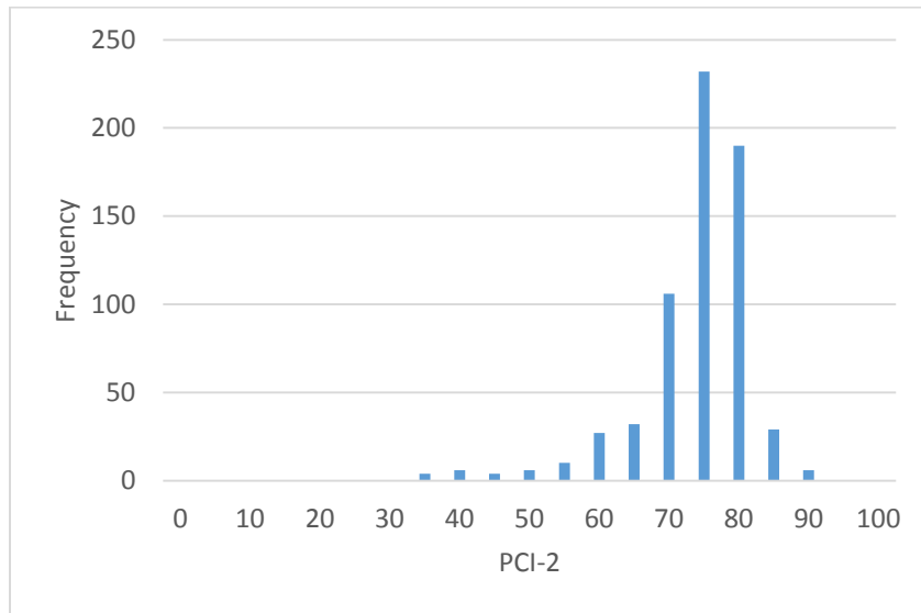
Figure 33. PCI-2 for PCC Type 1-Interstate
