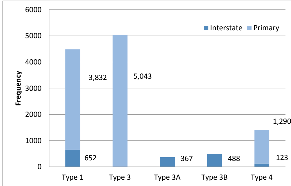
Figure 2. Frequency of data points based on pavement type used for Cracking, Riding, Rutting, and Faulting Indices
