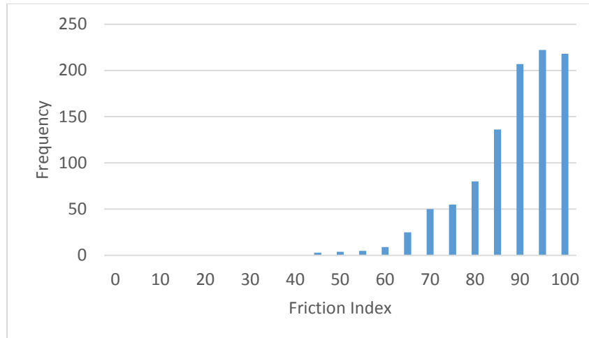
Figure 32. Friction Index for AC Type 4-Primary
