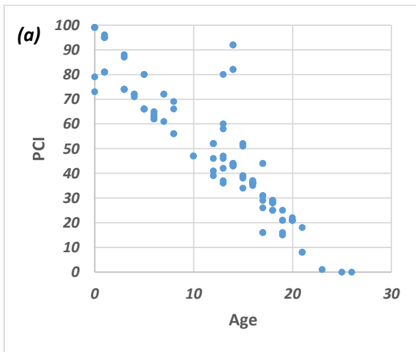
Figure 52. Deterioration of pavement condition by pavement age for AC Type 4-Interstate: (a) using PCI, (b) using PCI-2
