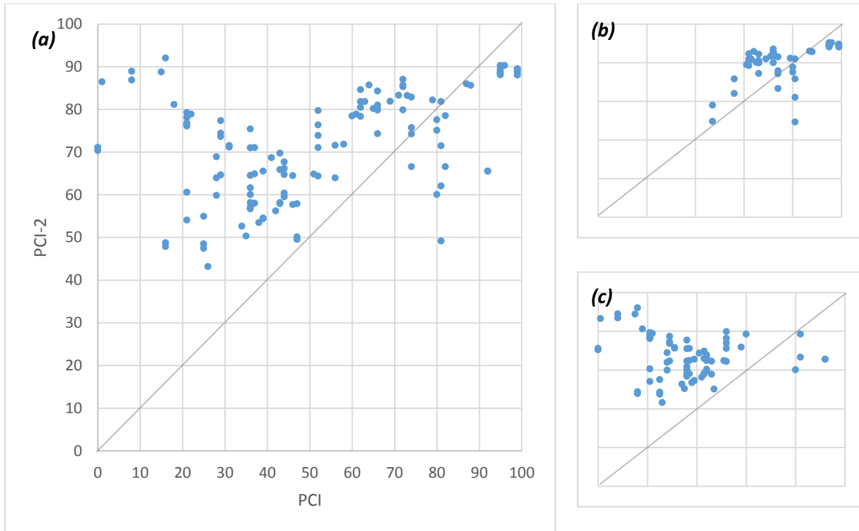
Figure 45. Comparison of PCI and PCI-2 for AC Type 4-Interstate: (a) complete data set, (b) sections less than 10 years old, (c) sections 10 to 25 years old
