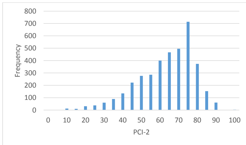
Figure 34. PCI-2 for PCC Type 1-Primary
