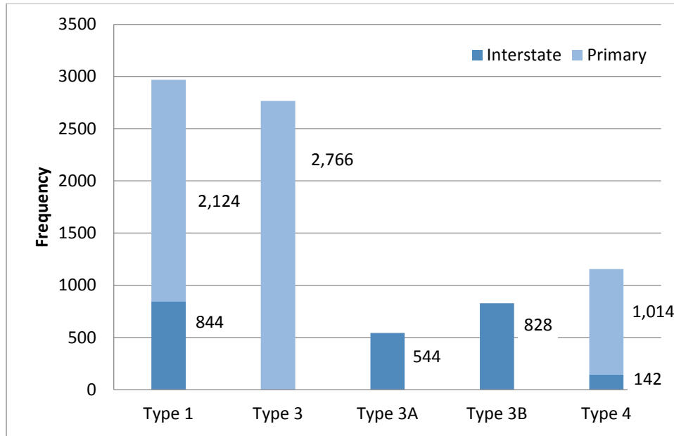
Figure 3. Frequency of data points based on pavement type used for Friction Index
