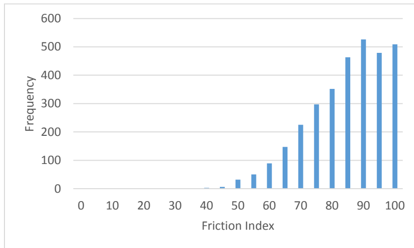
Figure 28. Friction Index for composite with asphalt surface Type 3
