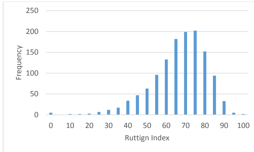
Figure 22. Rutting Index for AC Type 4-Primary
