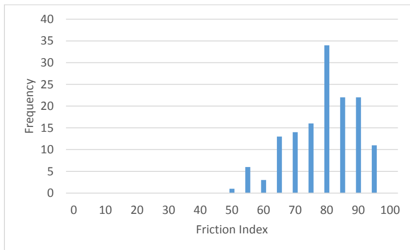
Figure 31. Friction Index for AC Type 4-Interstate
