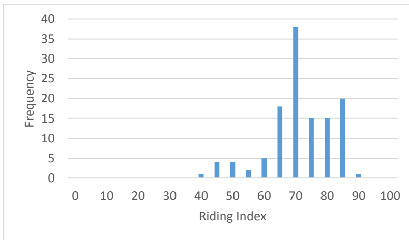
Figure 16. Riding Index for AC Type 4-Interstate
