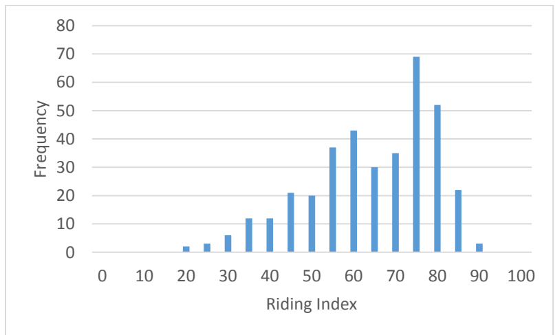
Figure 14. Riding Index for composite built on old jointed PCC Type 3A
