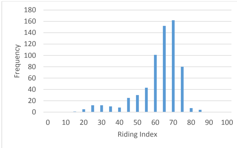
Figure 11. Riding Index for PCC Type 1-Interstate
