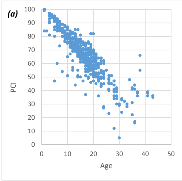
Figure 47. Deterioration of pavement condition by pavement age for PCC Type 1-Interstate: (a) using PCI, (b) using PCI-2
