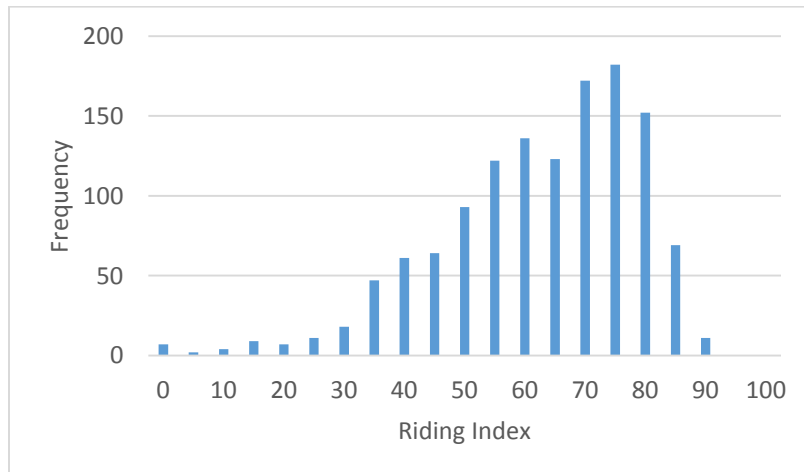
Figure 17. Riding Index for AC Type 4-Primary
