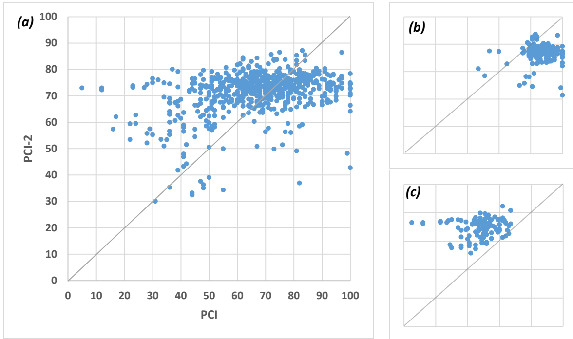
Figure 40. Comparison of PCI and PCI-2 for PCC Type 1-Interstate: (a) complete data set, (b) sections less than 10 years old, (c) sections 20 to 30 years old
