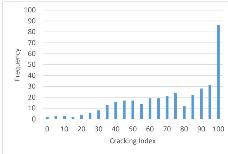
Figure 9. Cracking Index for composite built on old jointed PCC Type 3A
