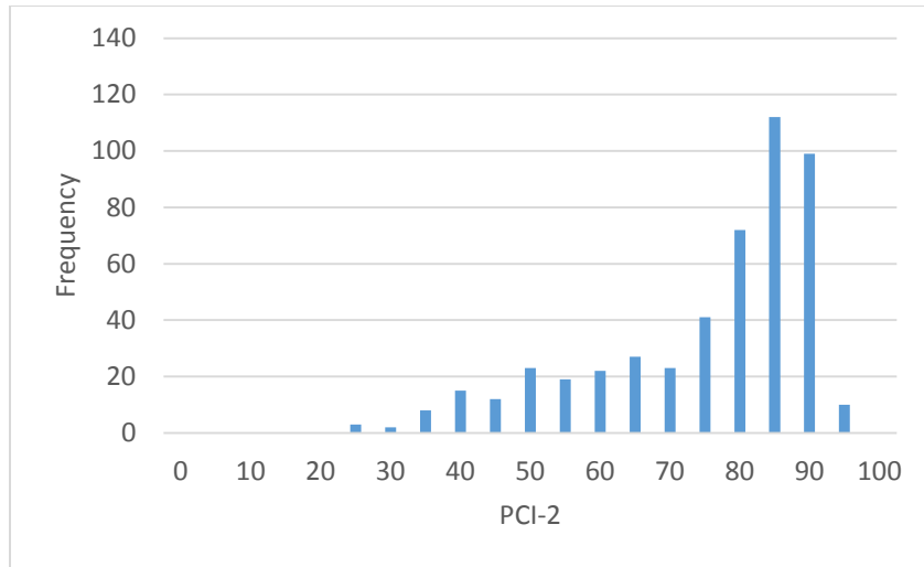
Figure 37. PCI-2 for Type 3B
