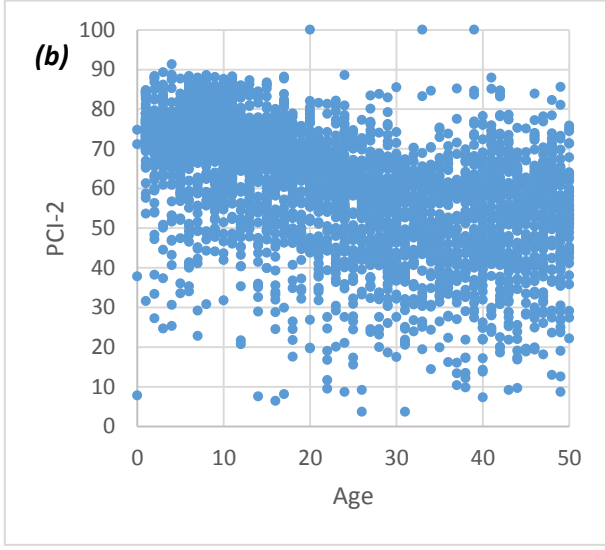
Figure 48. Deterioration of pavement condition by pavement age for PCC Type 1-Primary: (a) using PCI, (b) using PCI-2
