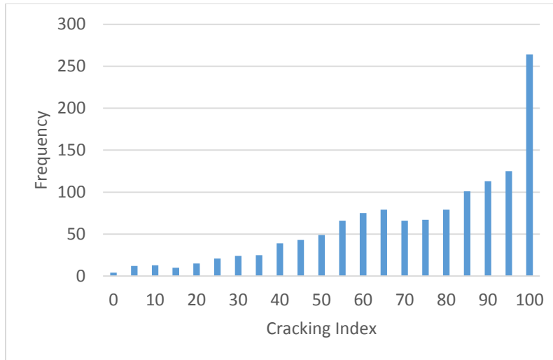
Figure 7. Cracking Index for AC Type 4-Primary
