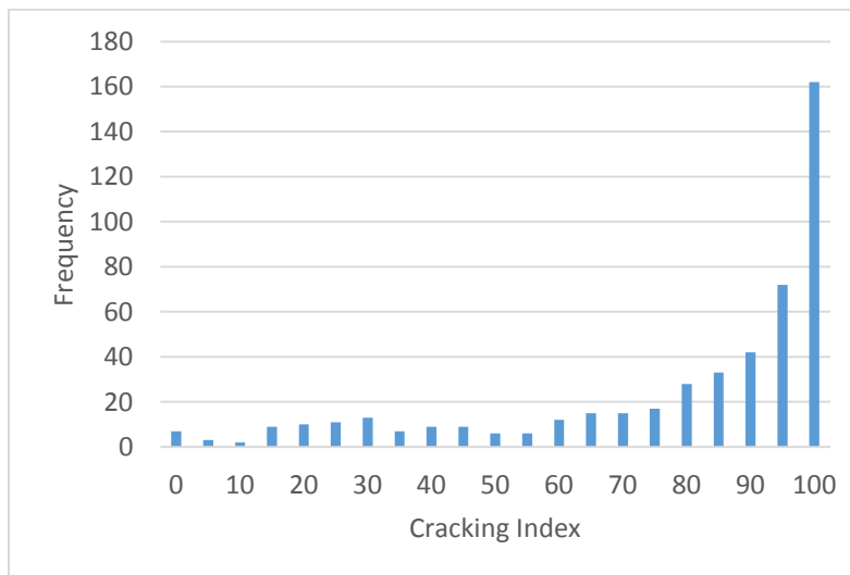
Figure 10. Cracking Index for composite built on old CRC Type 3B
