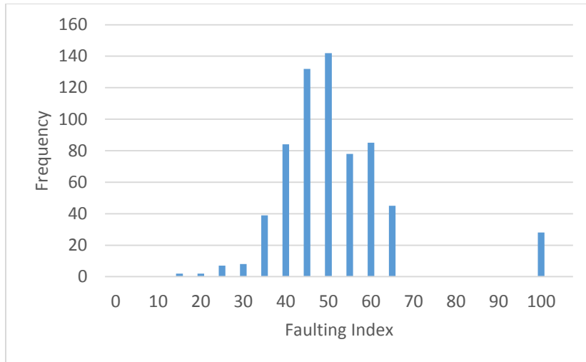
Figure 23. Faulting Index for PCC Type 1-Interstate
