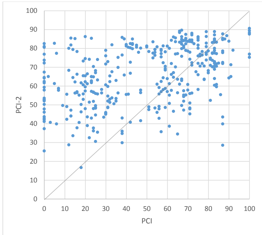
Figure 43. Comparison of PCI and PCI-2 for Type 3A composite built on old jointed PCC
