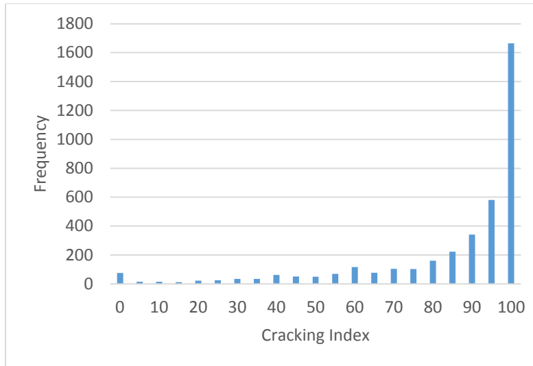
Figure 5. Cracking Index for PCC Type 1-Primary
