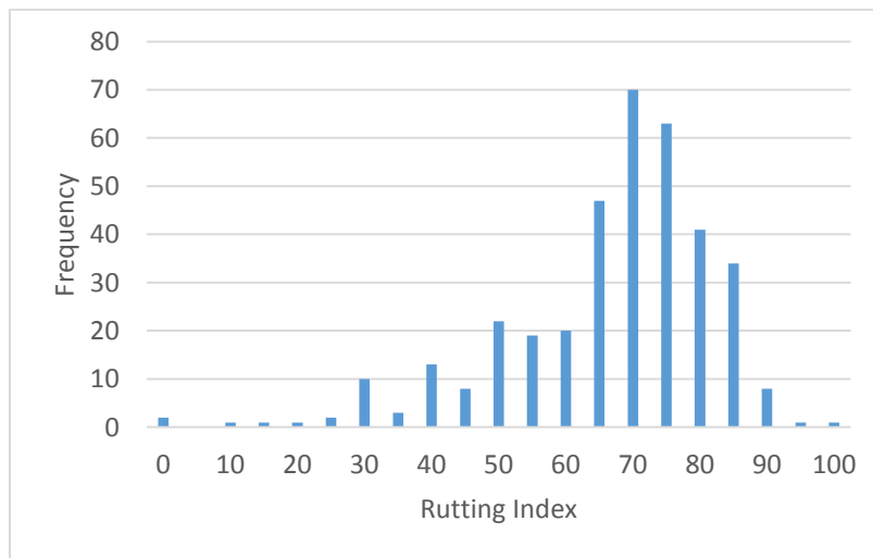
Figure 19. Rutting Index for composite built on old jointed PCC Type 3A
