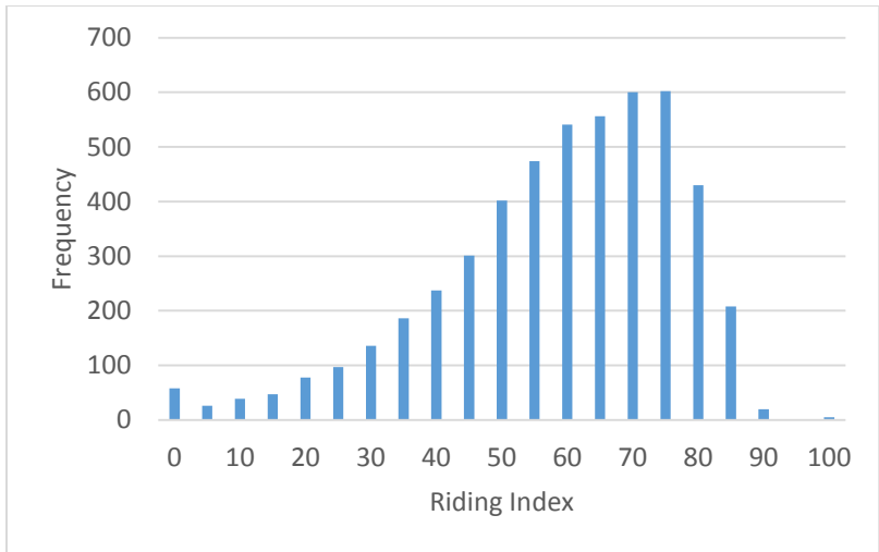
Figure 13. Riding Index for composite with asphalt surface Type 3
