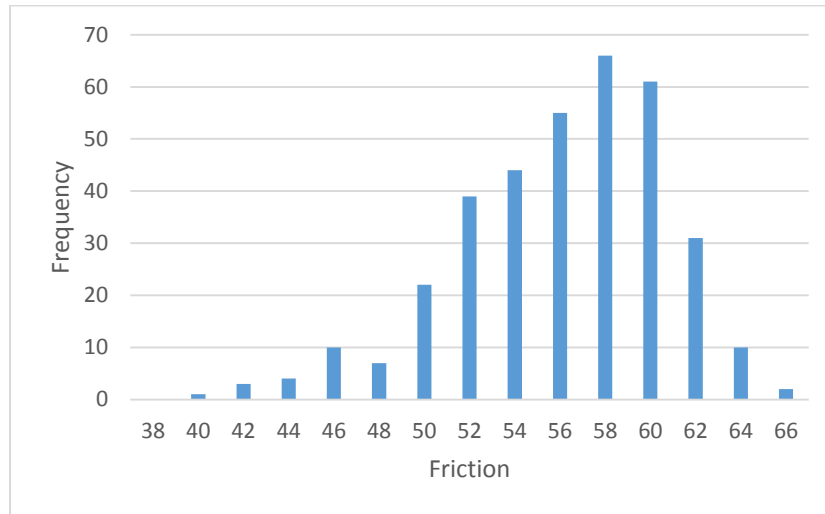
Figure 25. Friction Index for sections three years old or newer
