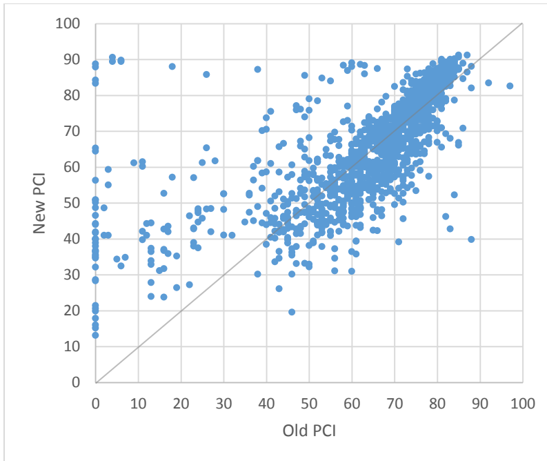
Figure 46. Comparison of PCI and PCI-2 for AC Type 4-Primary
