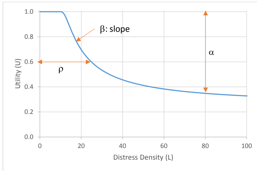
Figure 1. General shape of utility curves used for computing TxDOT pavement performance indices
