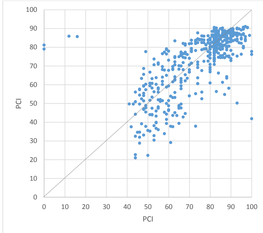
Figure 44. Comparison of PCI and PCI-2 for Type 3B composite built on old CRC
