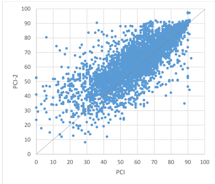
Figure 42. Comparison of PCI and PCI-2 for Type 3 composite with asphalt surface
