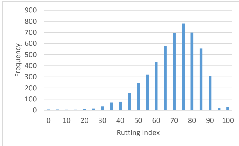
Figure 18. Rutting Index for composite with asphalt surface Type 3
