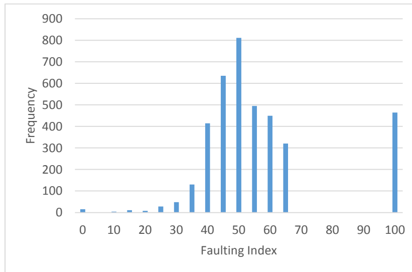
Figure 24. Faulting Index for PCC Type 1-Primary
