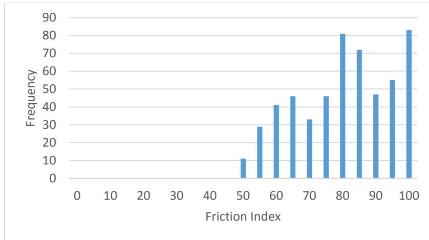
Figure 29. Friction Index for composite built on old jointed PCC Type 3A
