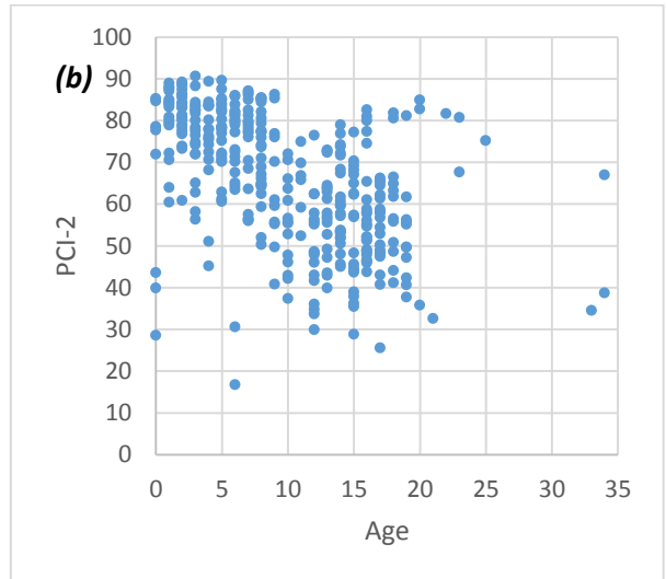
Figure 50. Deterioration of pavement condition by pavement age for Type 3A composite built on old jointed PCC: (a) using PCI, (b) using PCI-2
