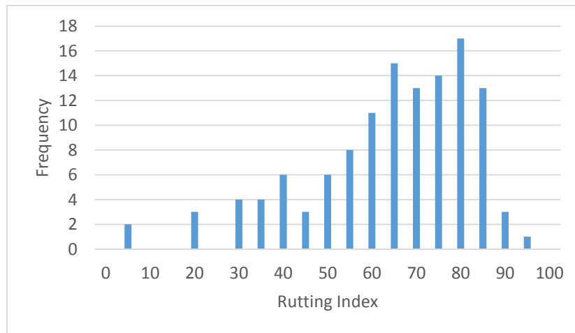
Figure 21. Rutting Index for AC Type 4-Interstate
