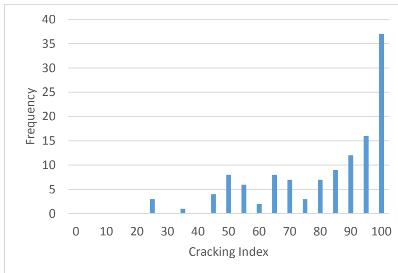
Figure 6. Cracking Index for AC Type 4-Interstate
