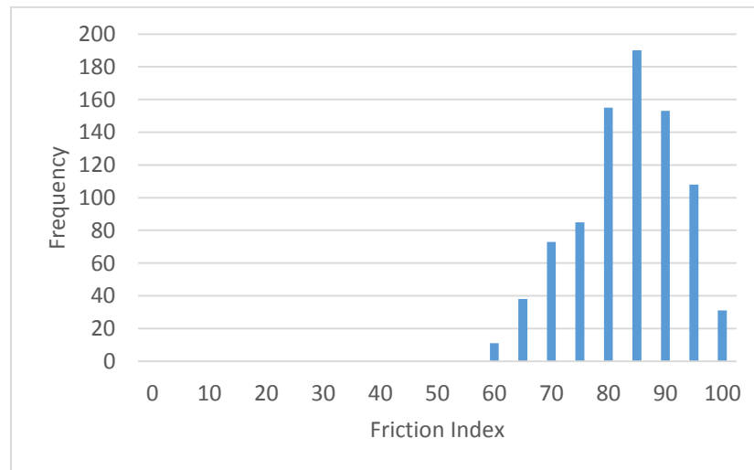
Figure 26. Friction Index for PCC Type 1-Interstate
