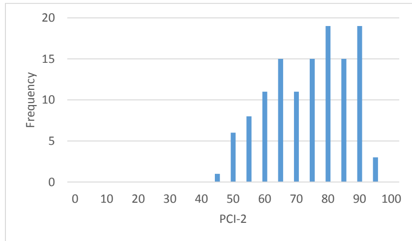
Figure 38. PCI-2 for AC Type 4-Interstate
