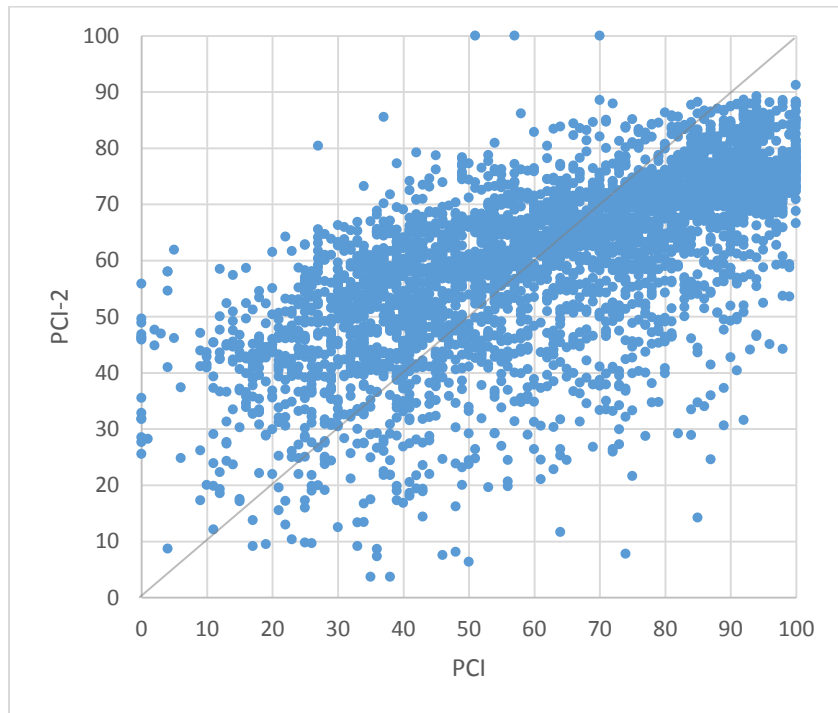
Figure 41. Comparison of PCI and PCI-2 for PCC Type 1-Primary
