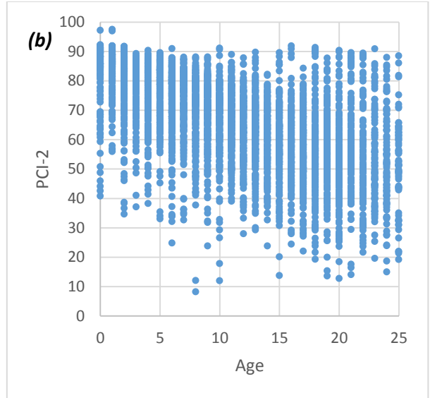
Figure 49. Deterioration of pavement condition by pavement age for Type 3 composite with asphalt surface: (a) using PCI, (b) using PCI-2
