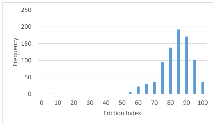
Figure 30. Friction Index for composite built on old CRC Type 3B
