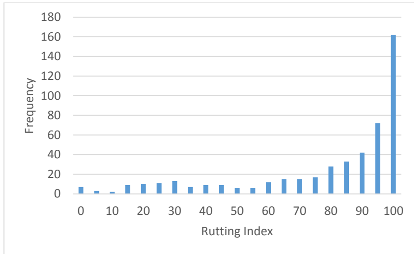
Figure 20. Rutting Index for composite built on old CRC Type 3B
