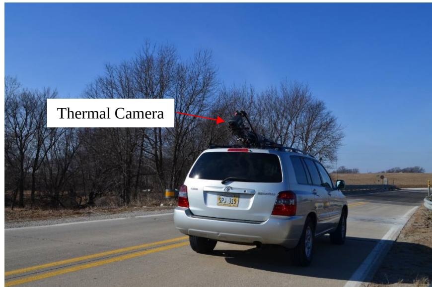
Figure 3.13. Thermal image scanning of Mud Creek Bridge using thermal camera mounted on a vehicle
