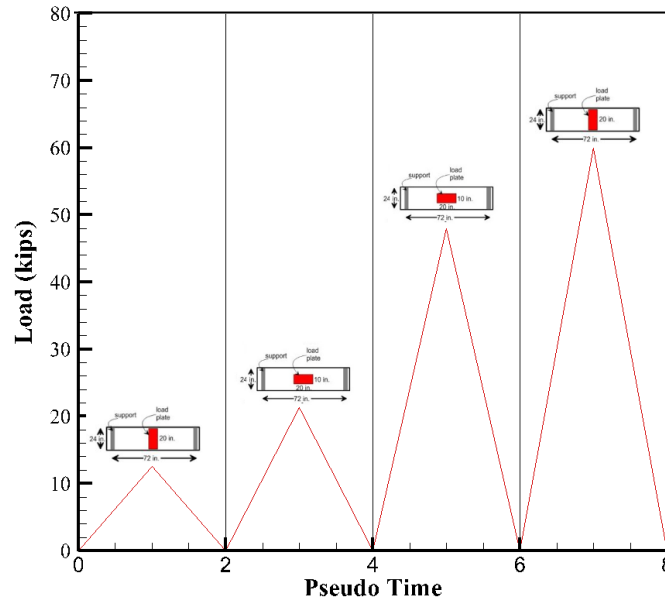
Figure 4.5. Load protocol for the tests
