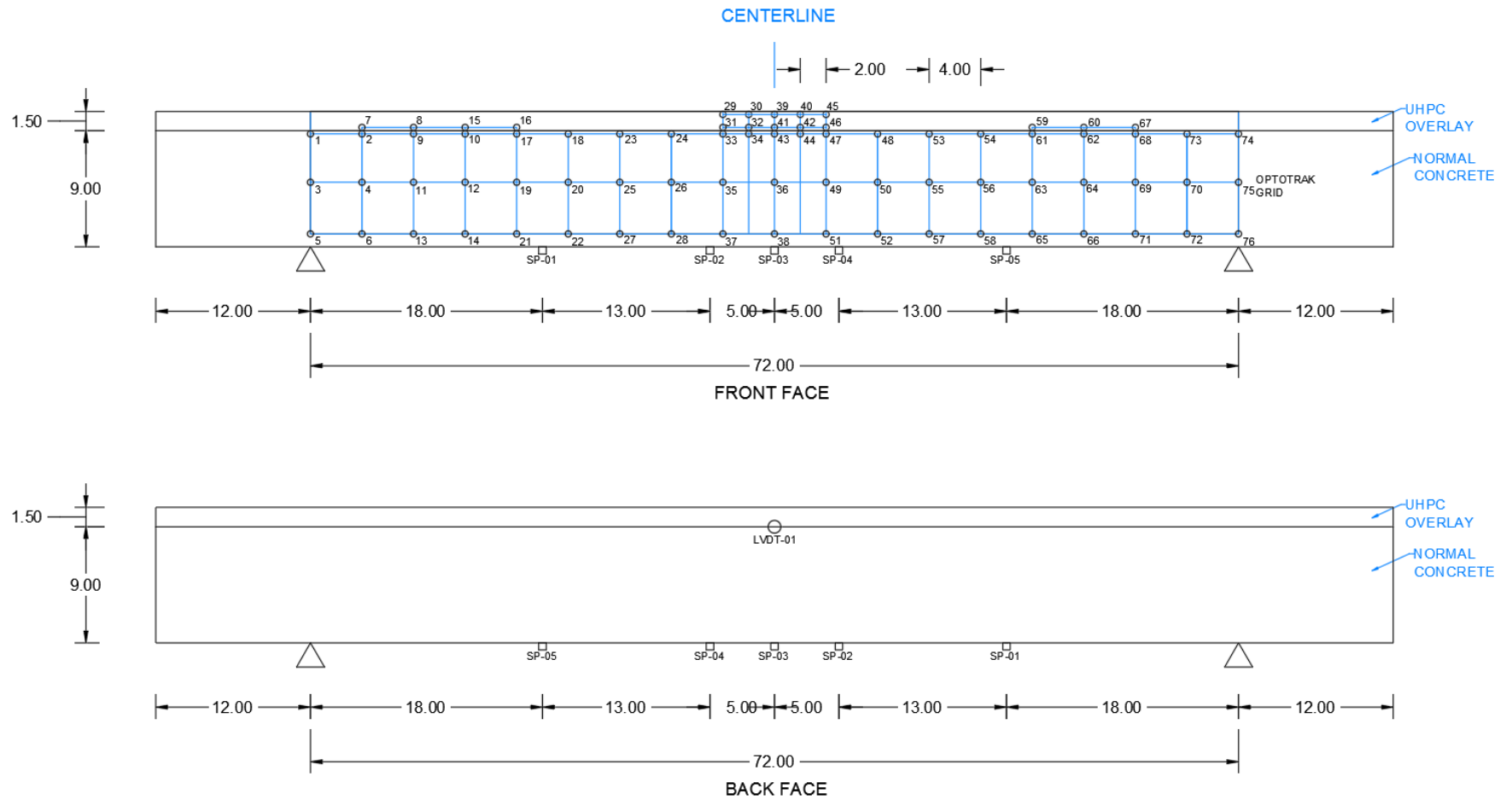
Figure 4.6. Instrumentation layout for Specimen OT
