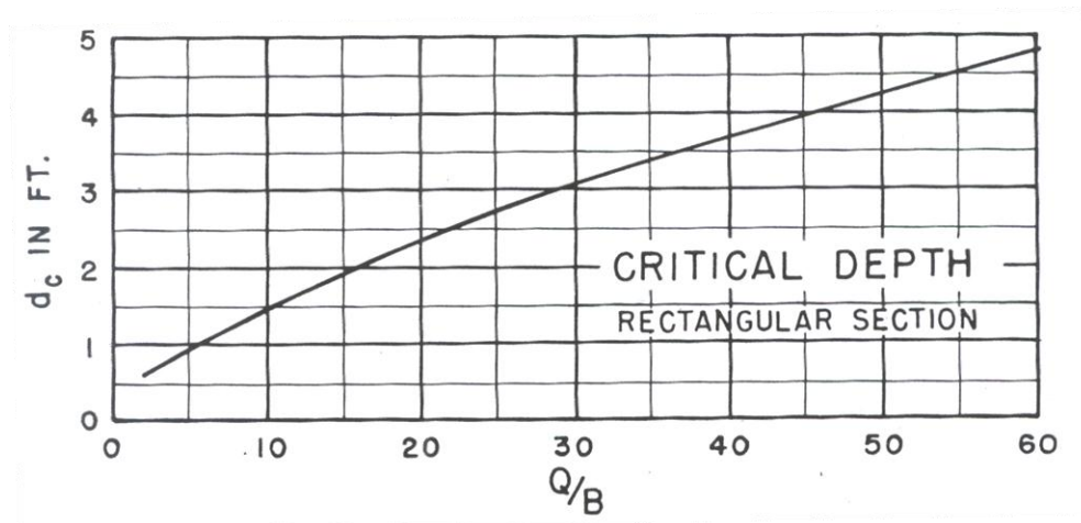
Figure 2E-2.04A: Critical Depth Box Culvert, Q/B = 0 to 60 cfs
