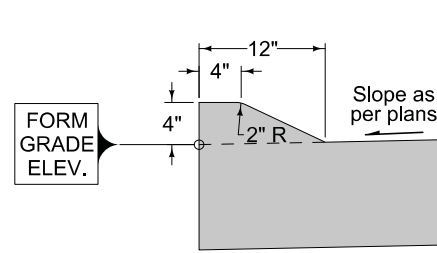
4" SLOPED CURB
