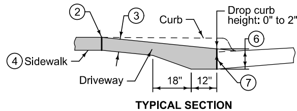
TYPICAL SECTION
