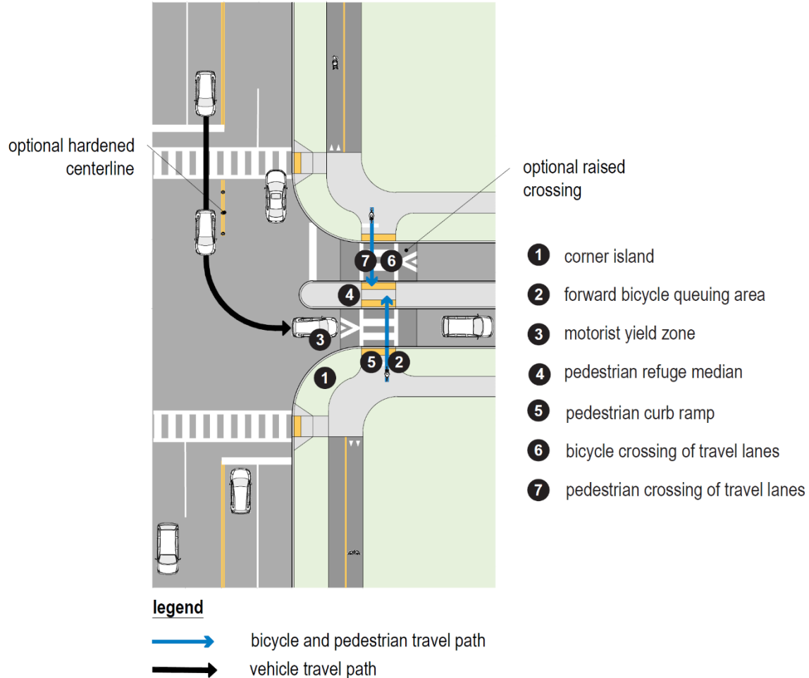
Figure 5M-1.05: Example of Hardened Centerline Applications with Flexible Delineators on the Departure Roadway and a Pedestrian Crossing Island on the Receiving Roadway
