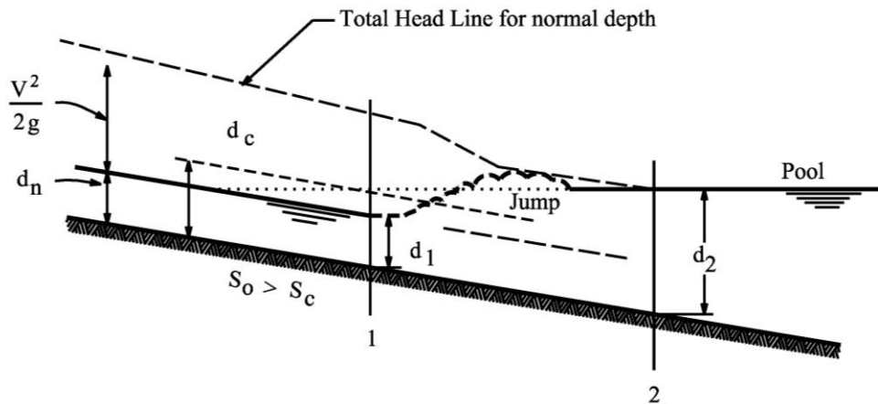
Figure 2F-2.05: Water Surface Profile Illustrating Hydraulic Jump
