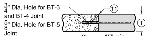
ABUTTING PAVEMENT JOINT - RIGID TIE (Drilled)
