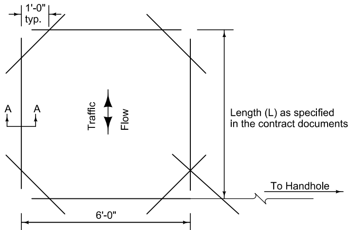
RECTANGULAR DETECTOR LOOP
