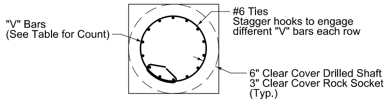
MAST ARM POLE FOUNDATION
