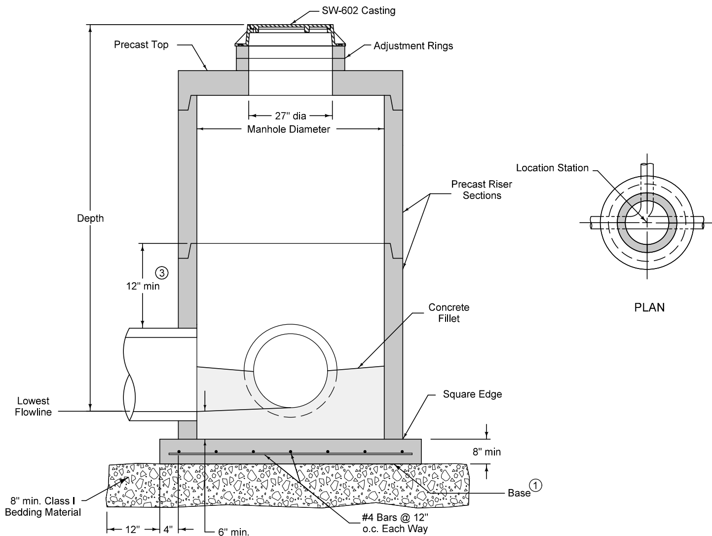
TYPICAL SECTION
