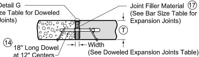
'ED', 'EE', 'EF' DOWELED EXPANSION JOINT
