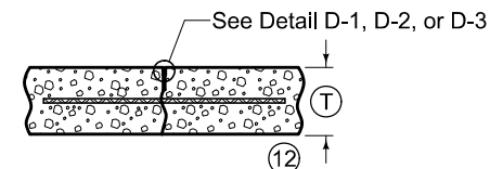
CONTRACTION JOINT
