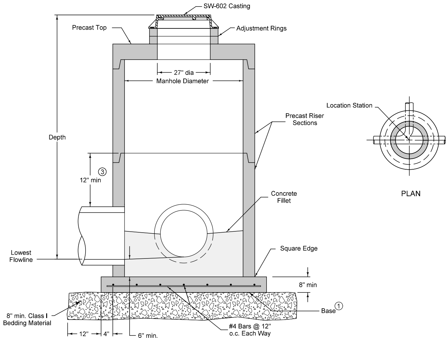
TYPICAL SECTION
