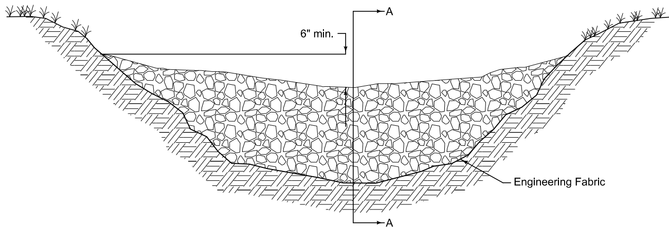
DITCH CROSS-SECTION
