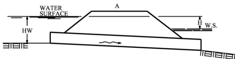
Figure 2E-2.02A: Inlet/Outlet Submerged
