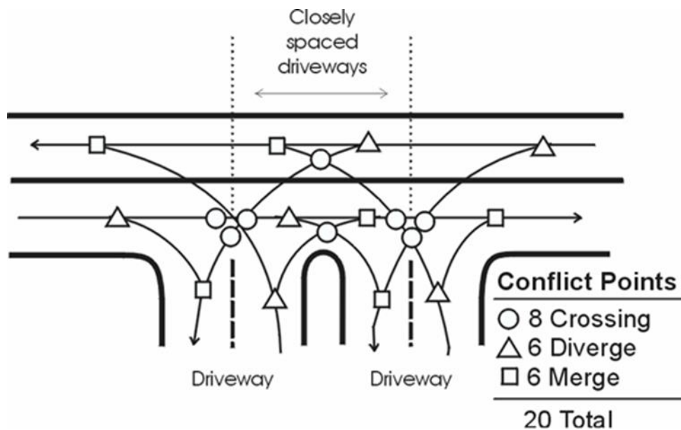
Figure 5L-3.03: Two Lane Undivided Roadway (Closely Spaced Entrances)
