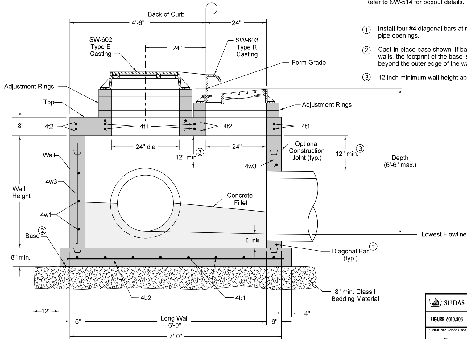
TYPICAL SECTION
