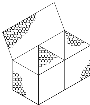
GABION ASSEMBLY
