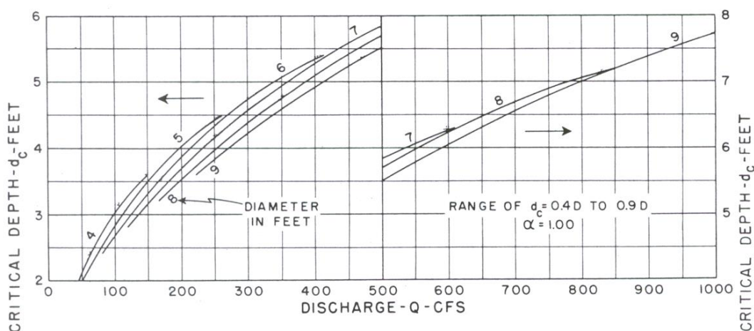
Figure 2E-2.03B: Critical Depth Circular Pipe, Discharge = 0 to 1000 cfs
