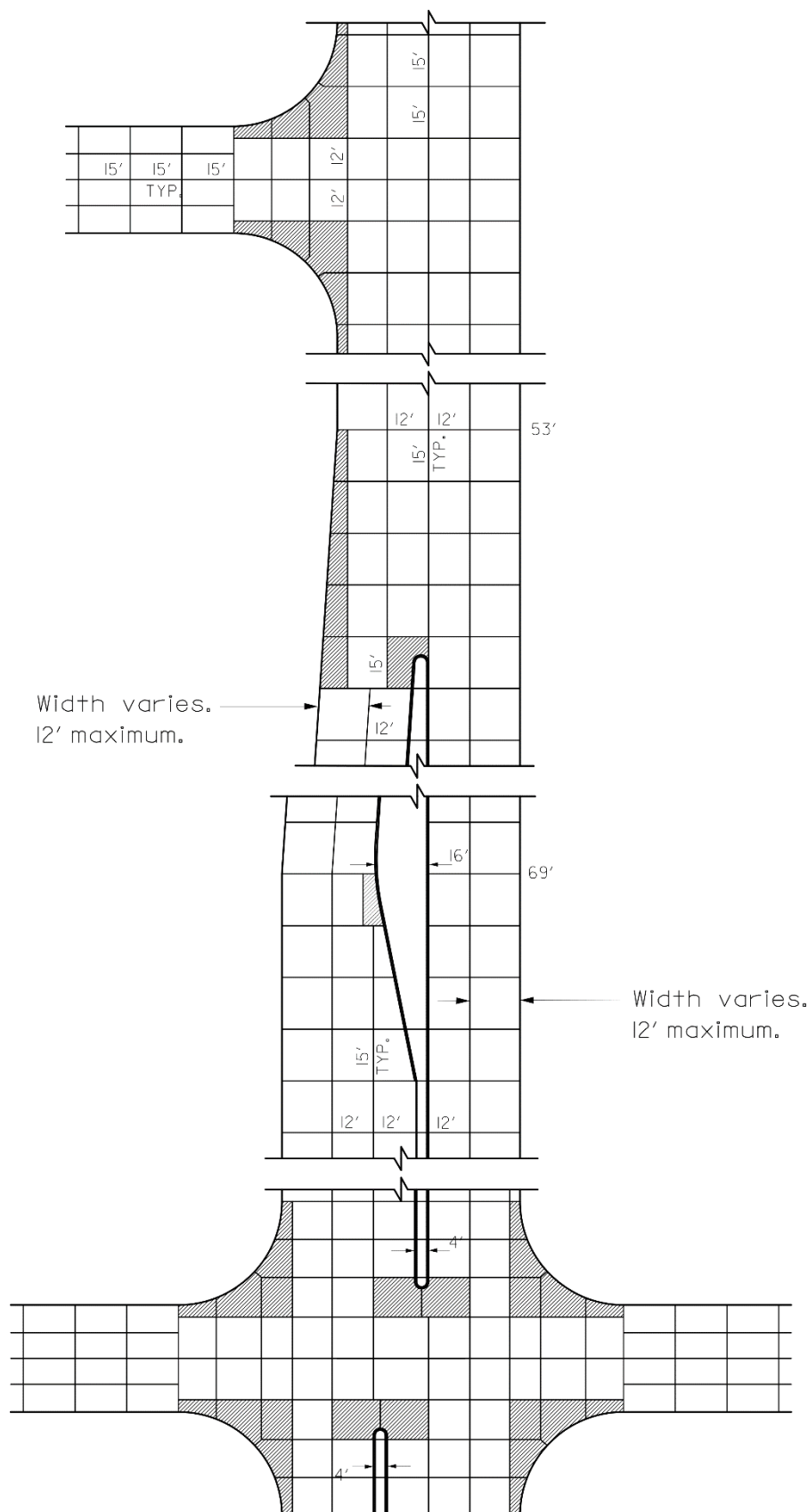
Figure 5G-3.11: Widening One Side - Four Lane to Five Lane
