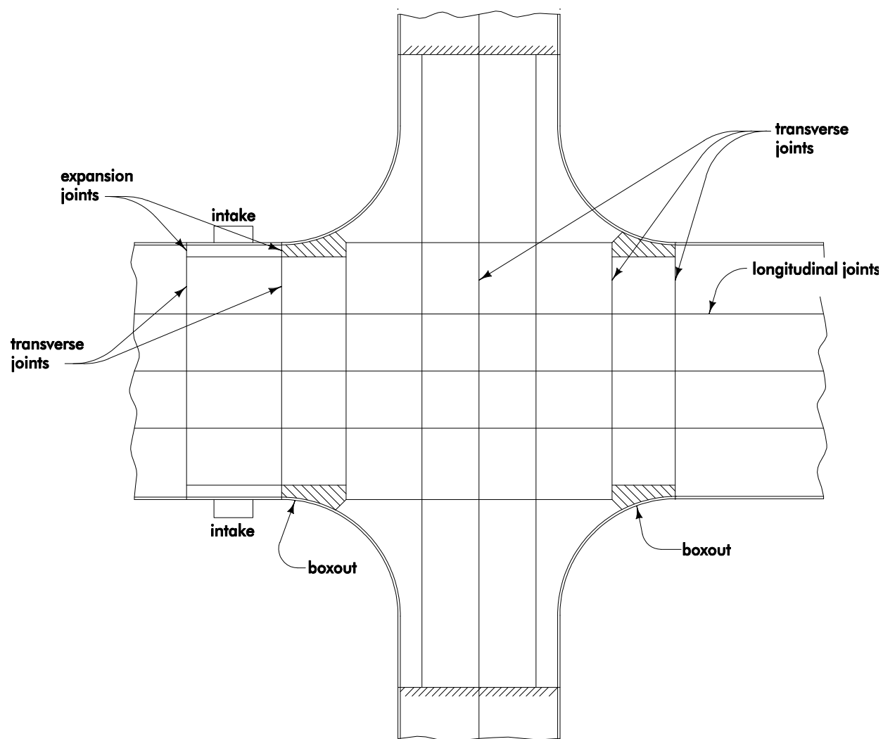
Figure 5G-3.01: Locating Predetermined and Difficult Joints
