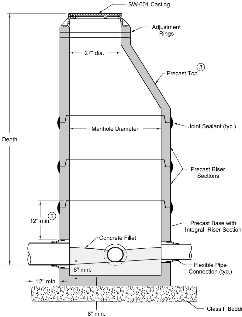
TYPICAL SECTION
