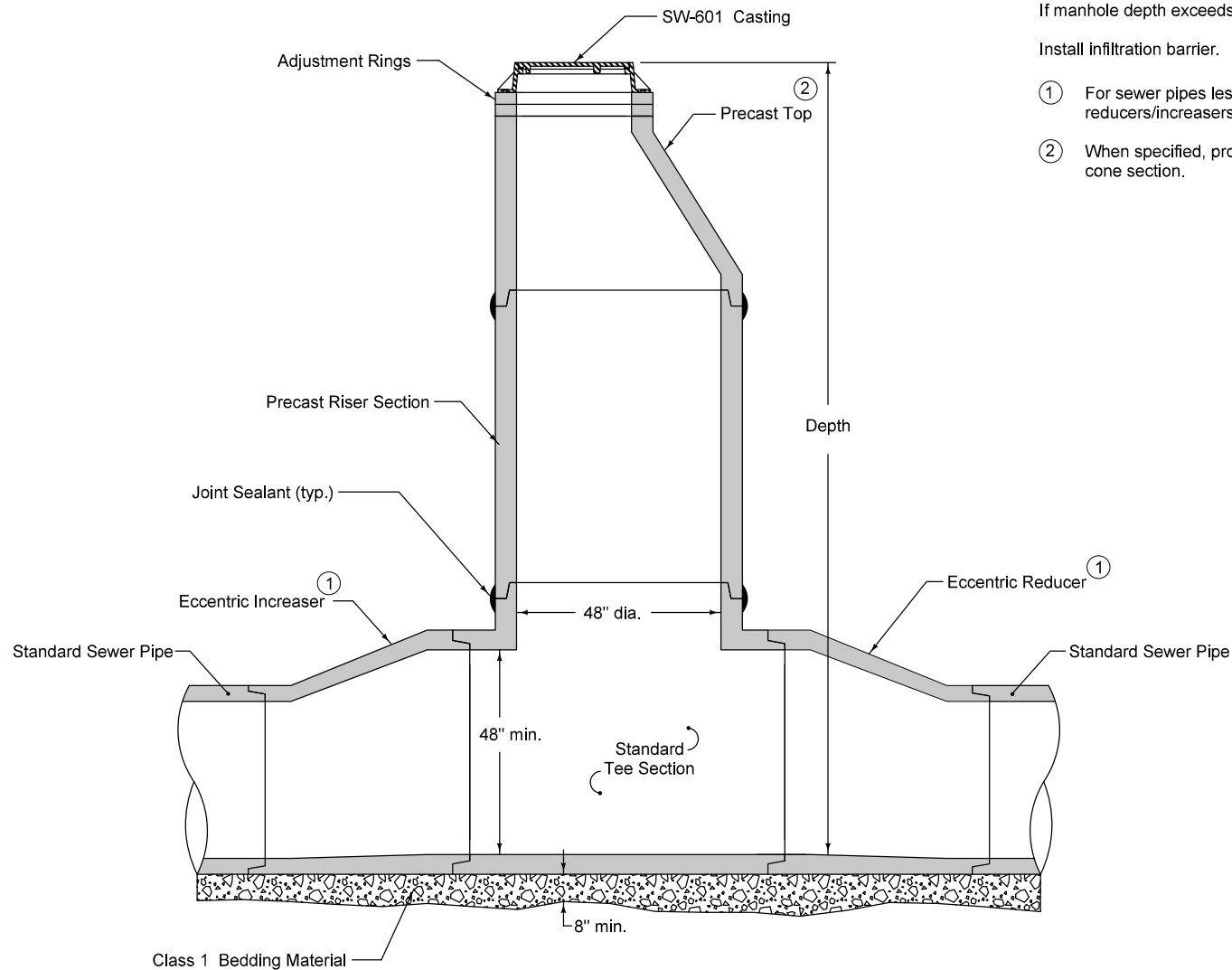
TYPICAL SECTION
