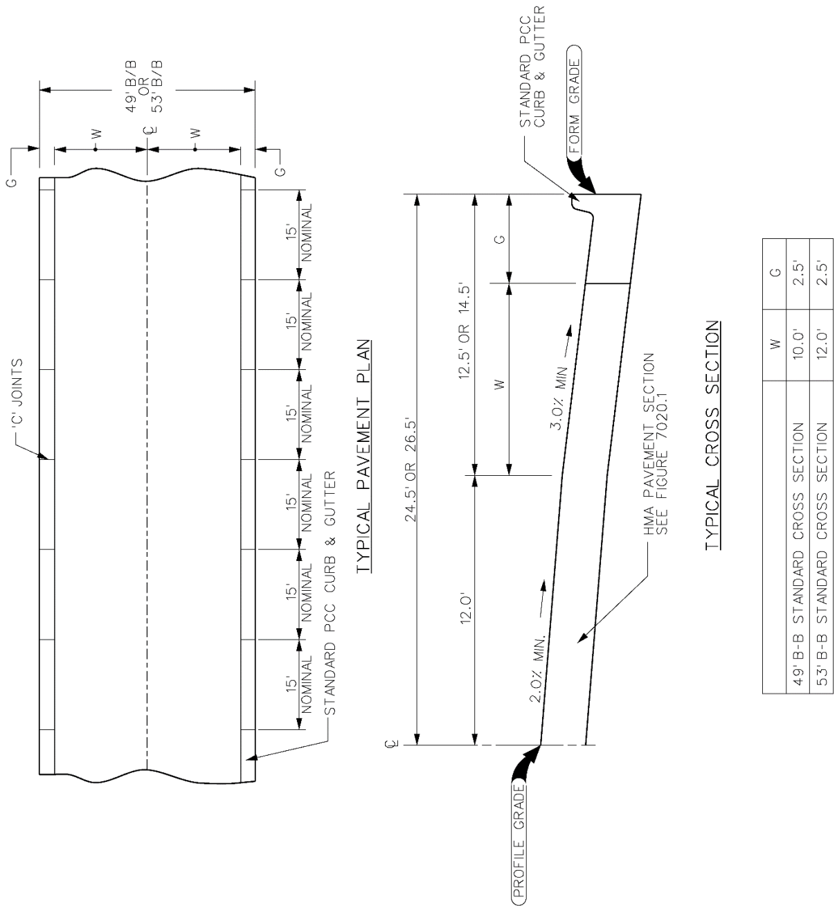
Figure 5G-2.12: 49' B/B and 53' B/B C&G/HMA Pavement
