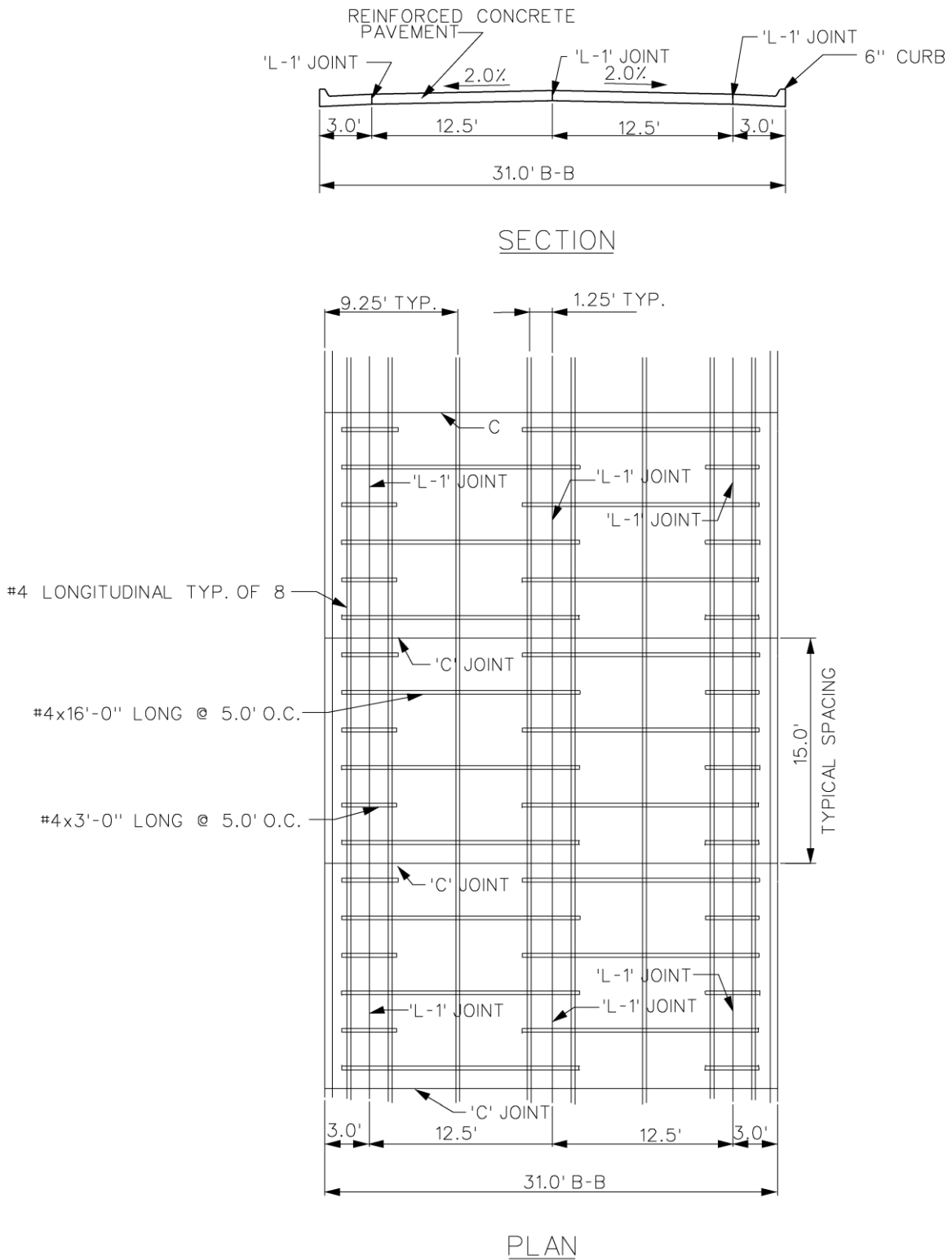
Figure 5G-2.10: Iowa Jointed Reinforced Pavement Detail - 31' Back-To-Back Street
