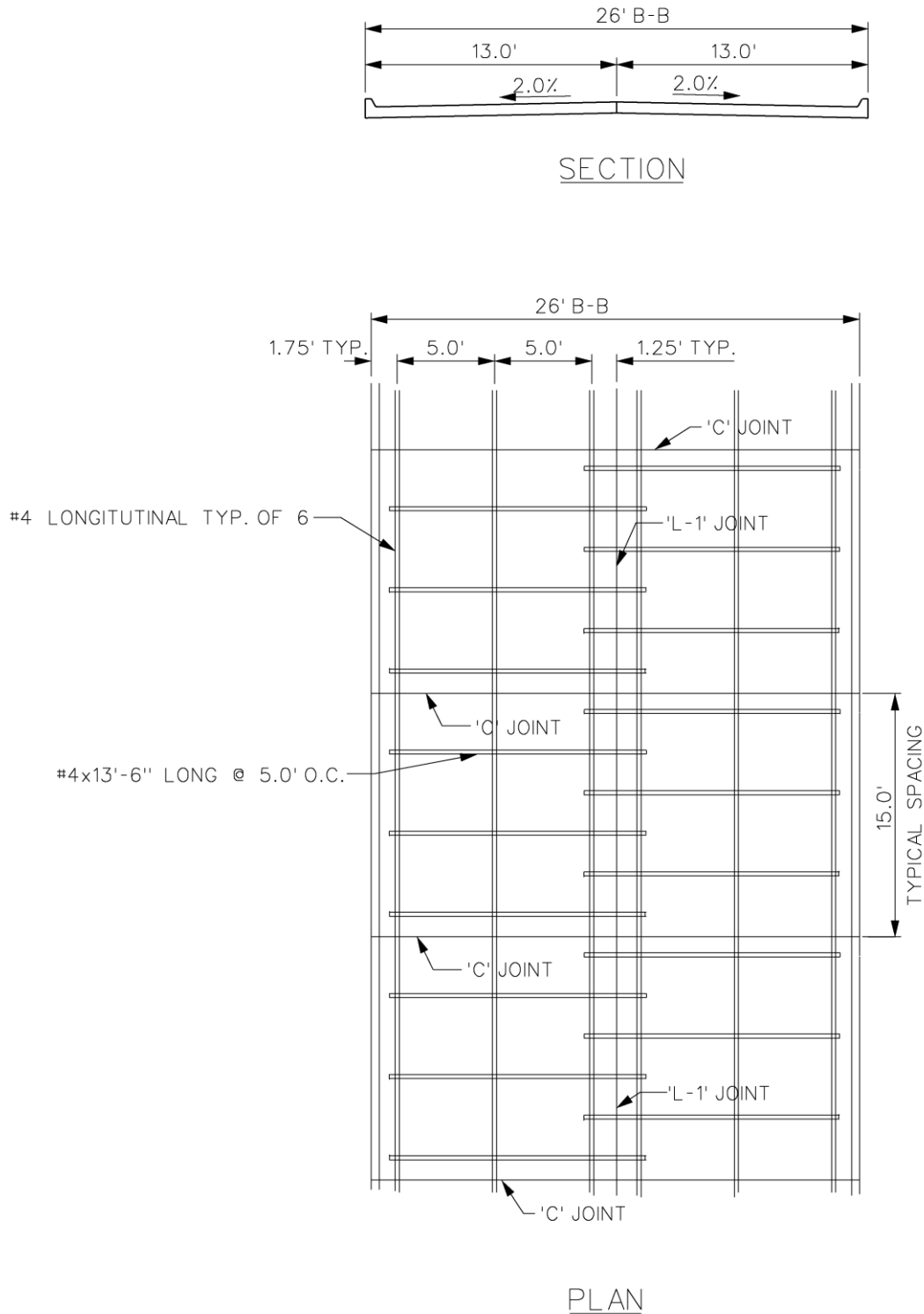
Figure 5G-2.09: Iowa Jointed Reinforced Pavement Detail - 26' Back-To-Back Street
