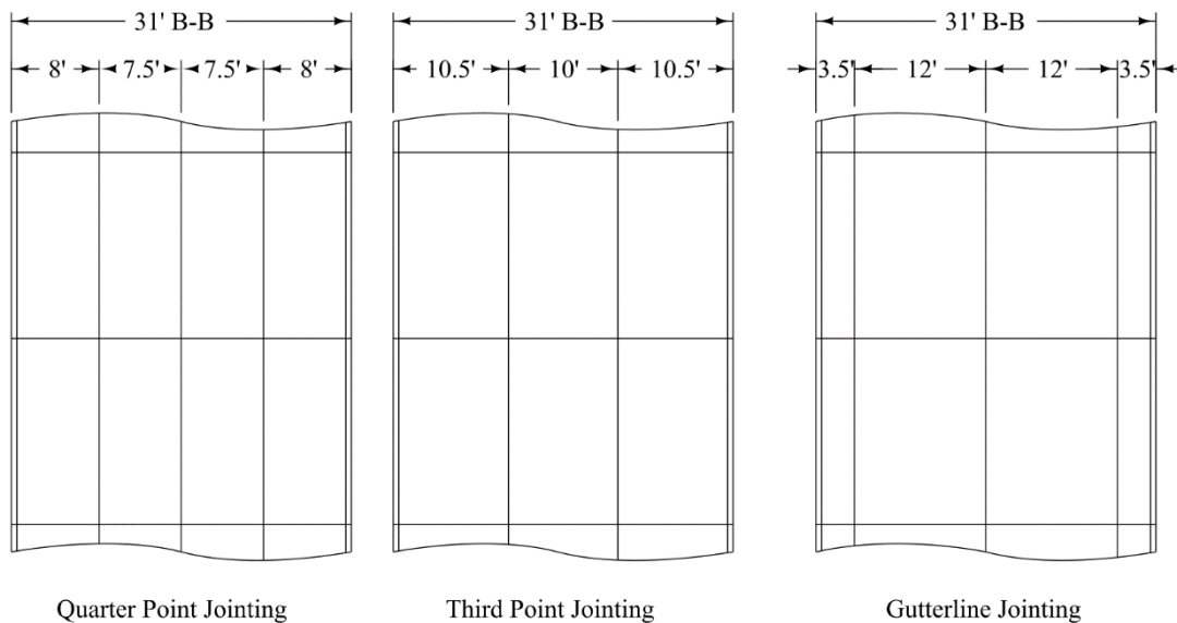
Figure 5G-2.05: 31 Foot B-B Pavements
