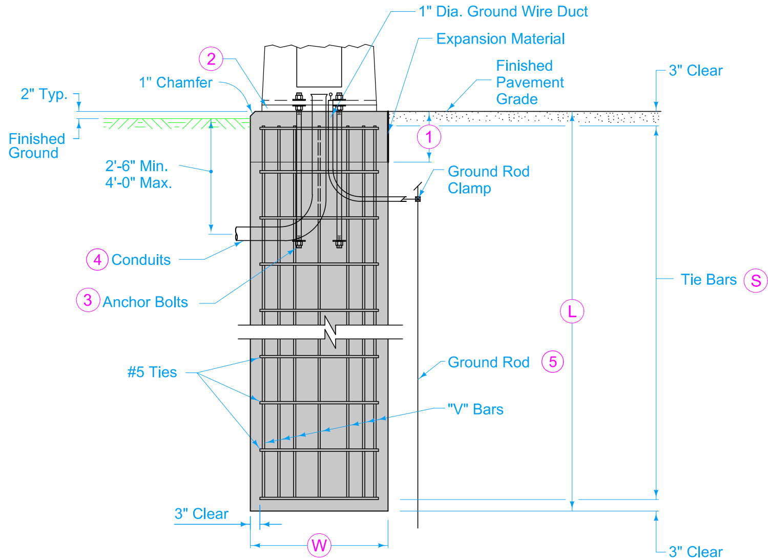
MAST ARM POLE FOUNDATION IN SOIL TYPE A FOUNDATION
